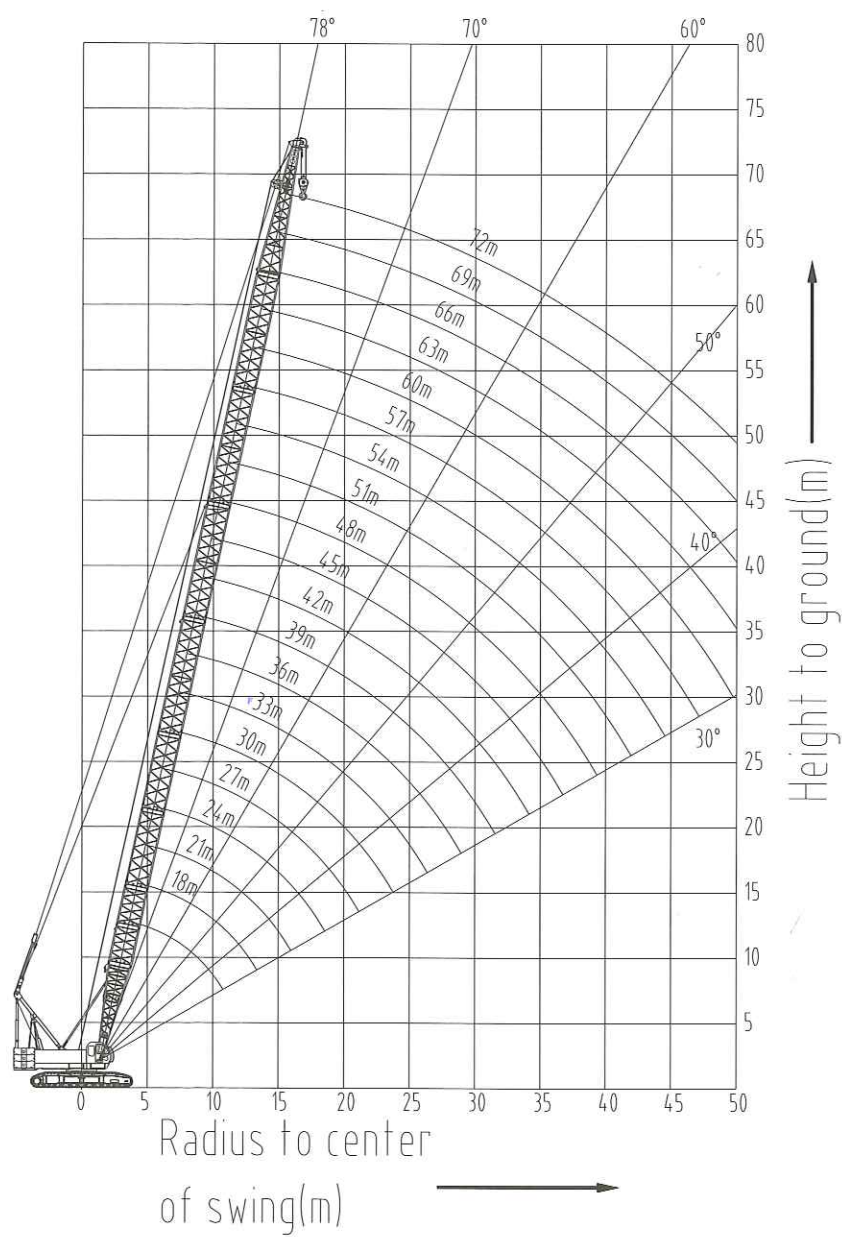
Curve of Lifting Height Scope
